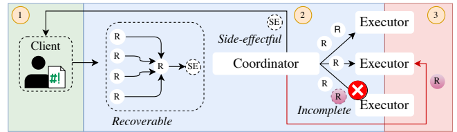
Fig. 1: FRAC TAL’s high-level workflow. FRAC TAL (1) isolates side-effectful regions from recoverable regions; (2) executes recoverable subgraphs on nodes, tracking locality, dependencies, progress, and health; (3) detects faults, re-scheduling the minimal set of unfinished subgraphs for re-execution.
